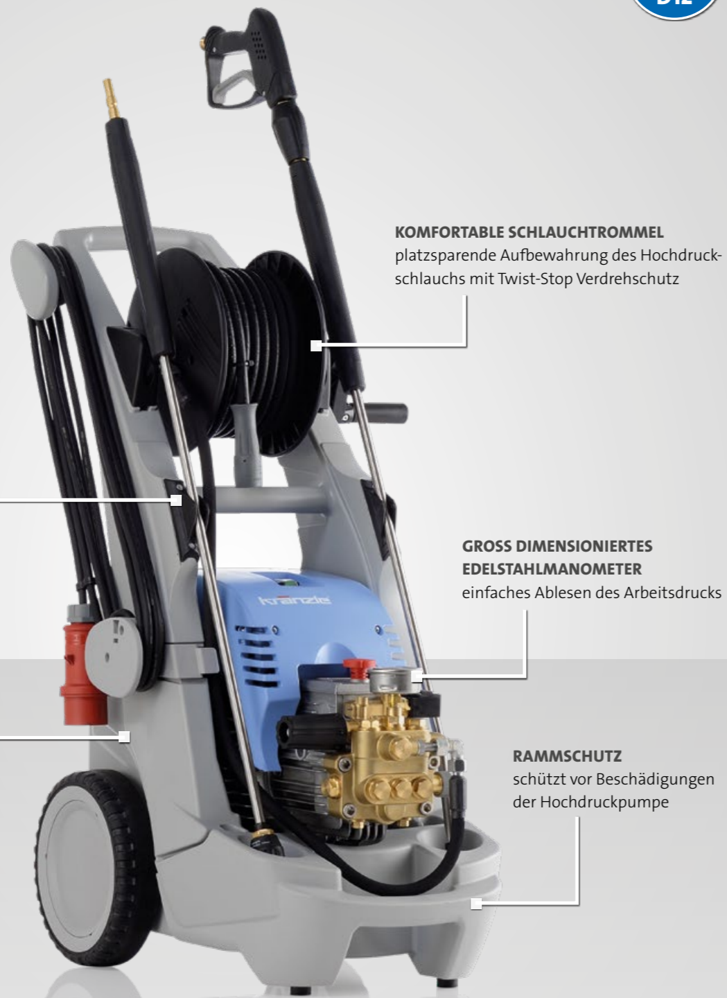
# 614050 bully 1000 TST
